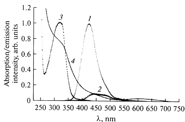
Fig. 2. Matching the (1, 2) luminescence and (3, 4) absorption spectra of (1, 3) NA and (2, 4) PPNA.
