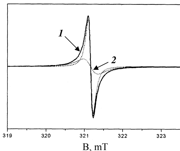
Fig. 3. A typical ESR spectrum of PPNA and its resolution on spectra of (1) long and (2) short polymer chains.
